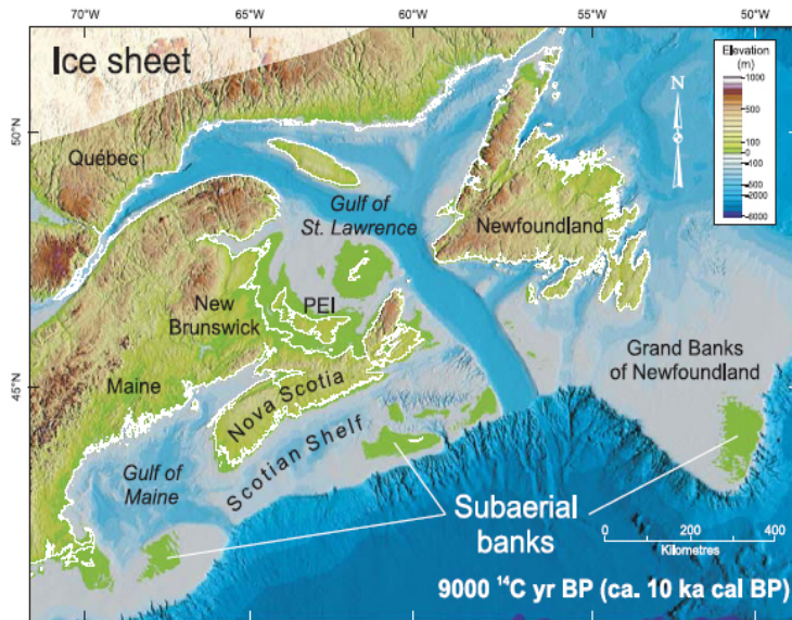
Figure 7. Palaeogeography of Atlantic Canada at 9000 ^{14}\text{C} yr BP (from Shaw et al. 2002) (ka cal BP: calibrated ^{14}\text{C} age, in thousands of years before present). At that time, islands ('subaerial banks') existed in the southern Gulf of Maine, on the Scotian Shelf and on the Grand Banks. Prince Edward Island (PEI) was part of the broad subaerial region extending from Nova Scotia and New Brunswick north into the Gulf of St. Lawrence.
